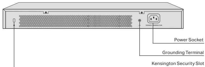
Figure 1-6 Rear Panel
