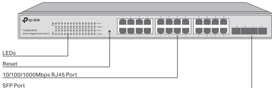
Figure 1-2 Front Panel of T1600G-28TS
