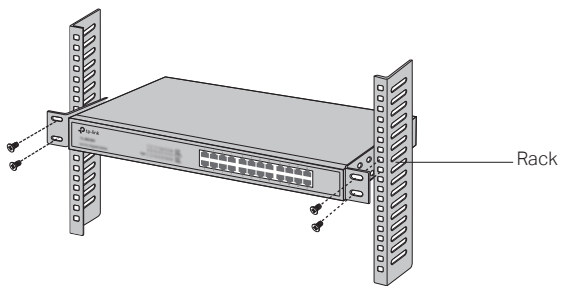
Figure 2-9 Rack Installation
