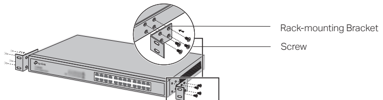
Figure 2-8 Bracket Installation
