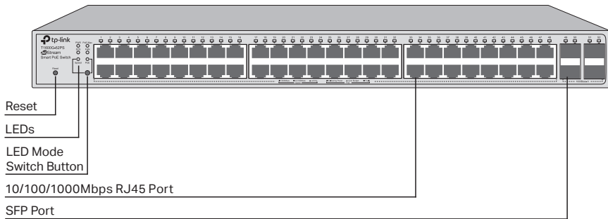
Figure 1-5 Front Panel of T1600G-52PS
