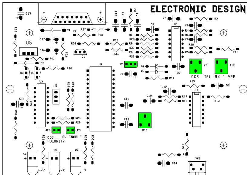
EDM-3 Layout
