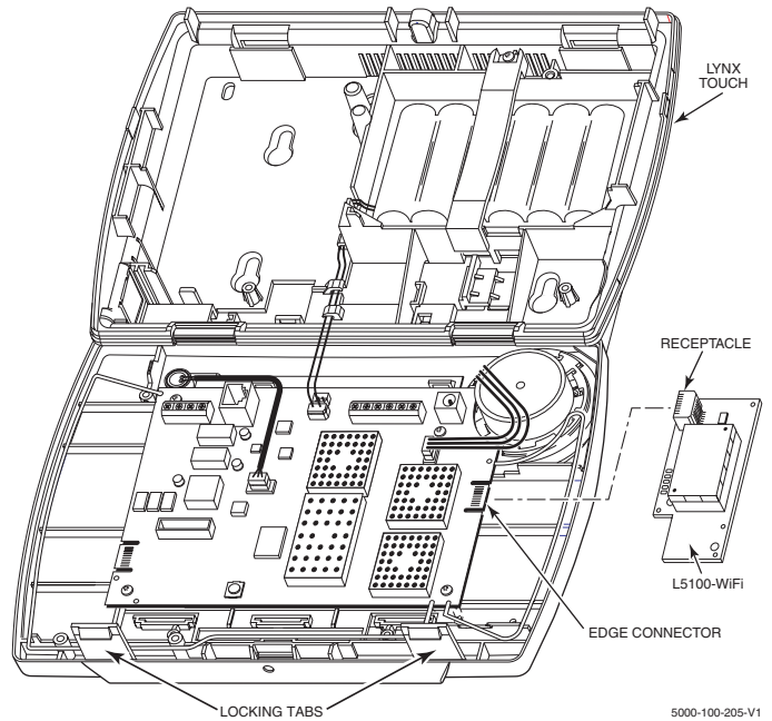
Figure 2. Installing the L5100-WiFi Communications Module
