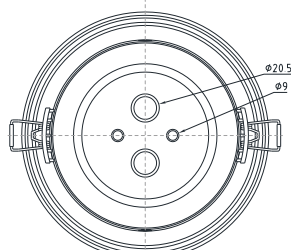
LM2-PCP06B
