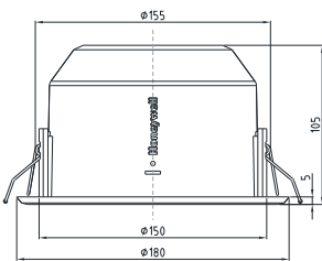
LM2-PCP06B
