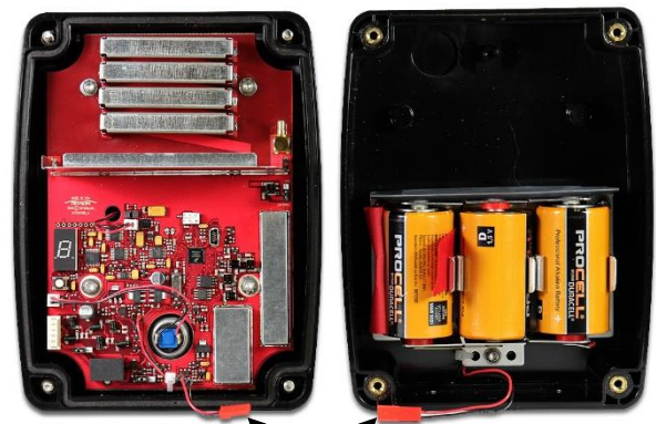
Q-Series power cable disconnected during battery installation
