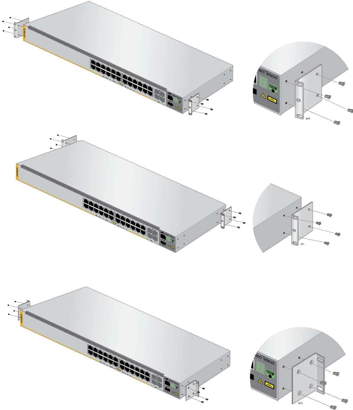
Figure 19. Attaching the Equipment Rack Brackets
