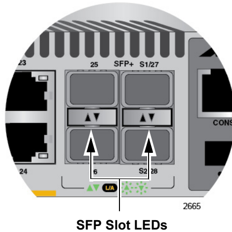
Figure 12. SFP+ Slot LEDs
