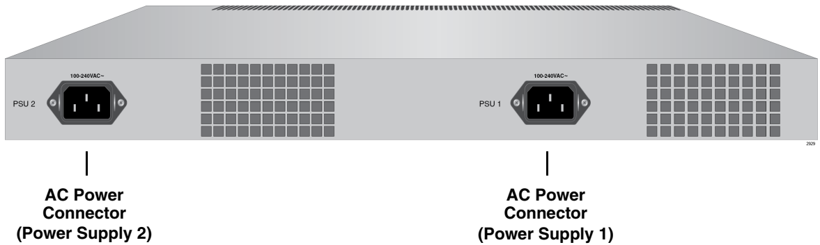
Figure 4. Back Panel of the AT-x510-28GPX and AT-x510-52GPX Switches
