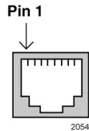
Figure 59. RJ-45 Socket Pin Layout (Front View)
