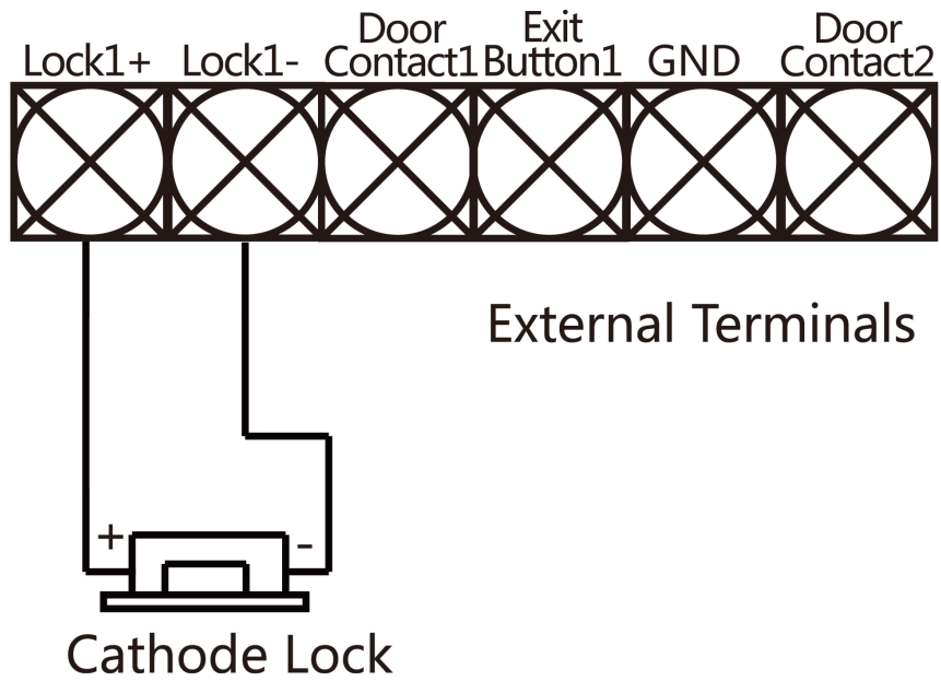
Figure 5-6 Wiring Diagram of Cathode Lock
