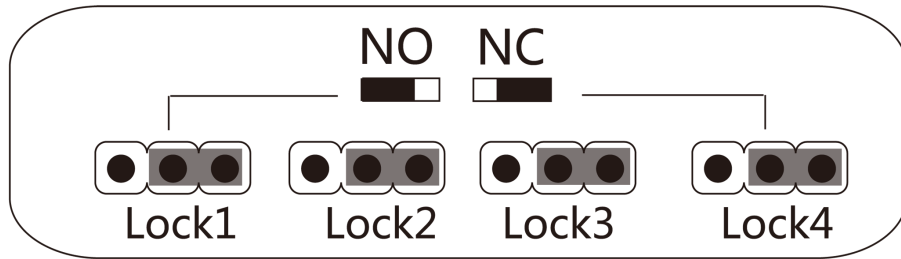
Figure 6-4 NC Status
