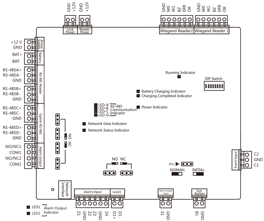
Figure 3-1 Single-Door Access Controller Main Board
